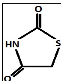
Fig 1: Thiazolidine-2, 4 - dione
